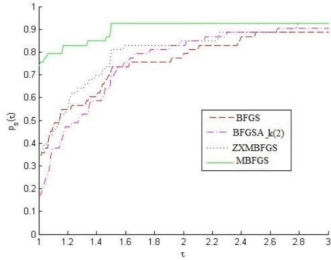
Figure 1: The Dolan-Moré performance profiles using number of function evaluations.
