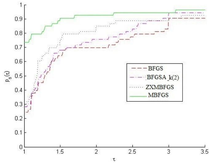
Figure 2: The Dolan-Moré performance profiles using number of iterations.
