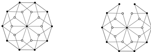
Figure 1: An illustration of Mycielski graphs \mu(C_{10}) (left) and \mu(P_{10}) (right)
