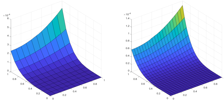
Figure 3: The graphs of error functions e_{10}(s), s = (s_1, s_2, 1) \in I_2(10) and e_{20}(s), s = (s_1, s_2, 1) \in I_2(20)
